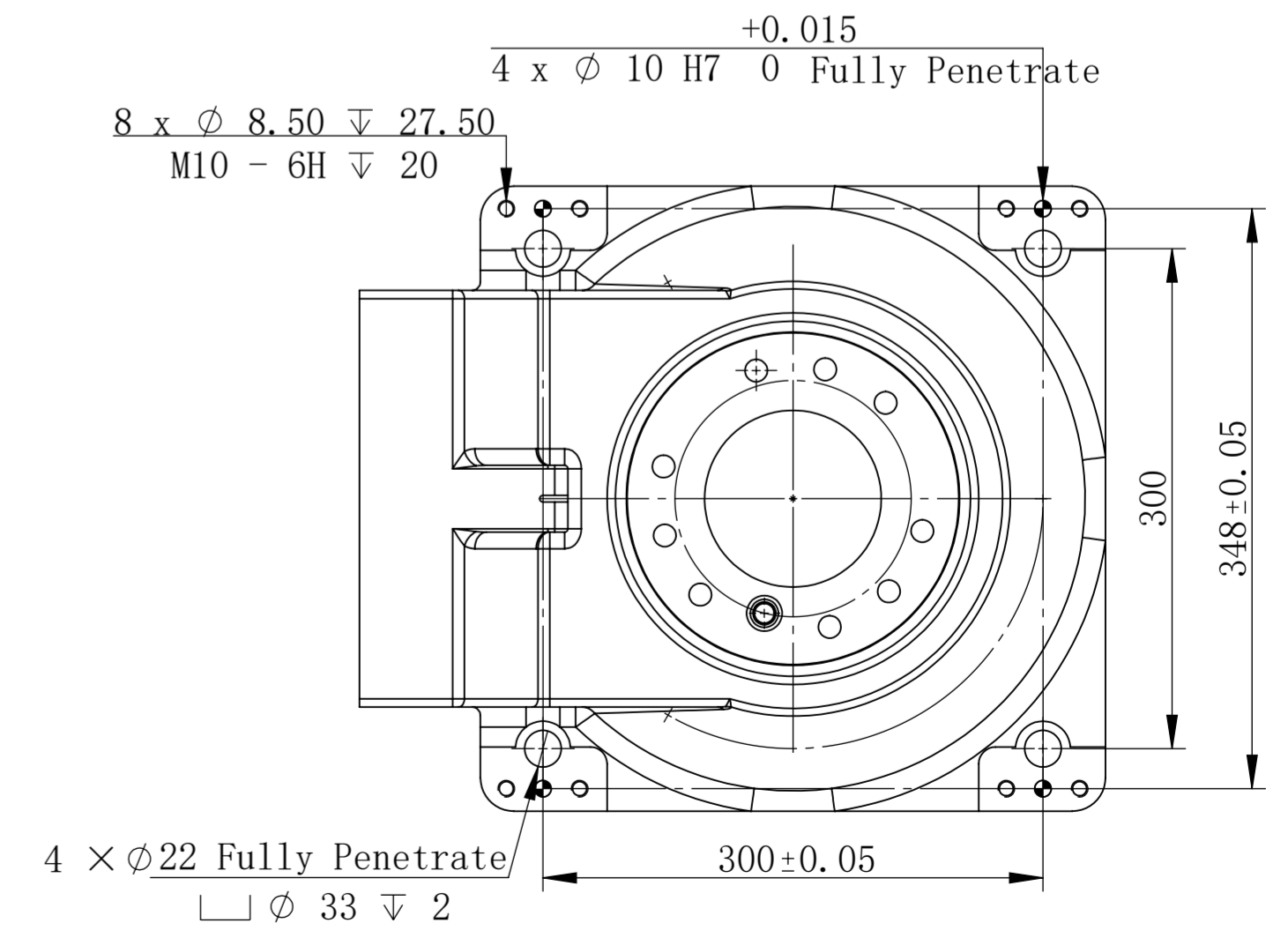
Base Installation Diagram
