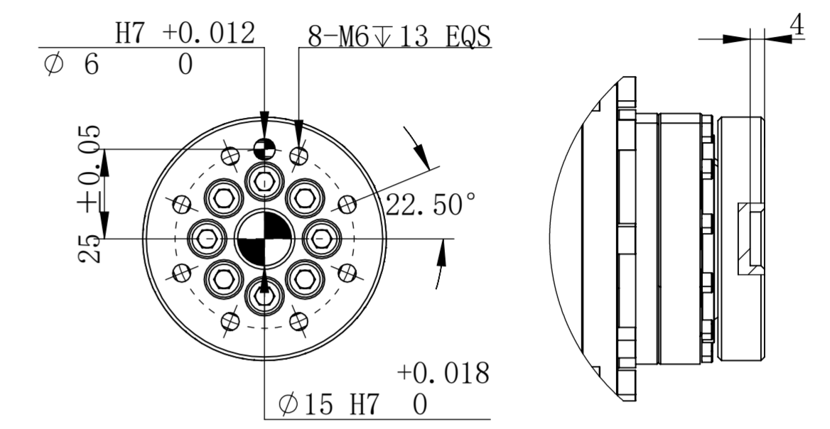
Base Installation Diagram
