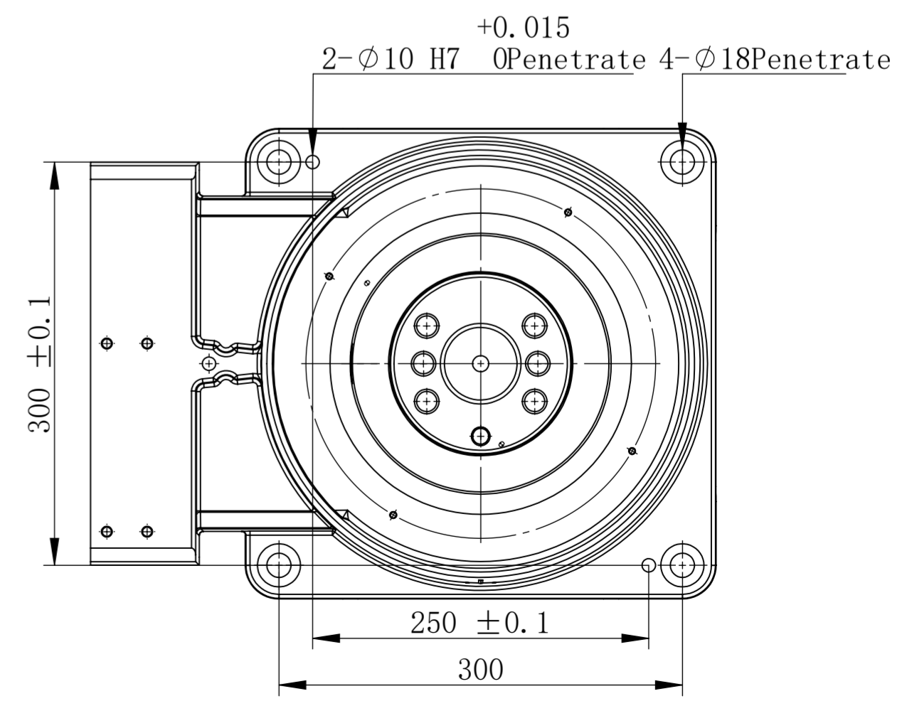
Base Installation Diagram
