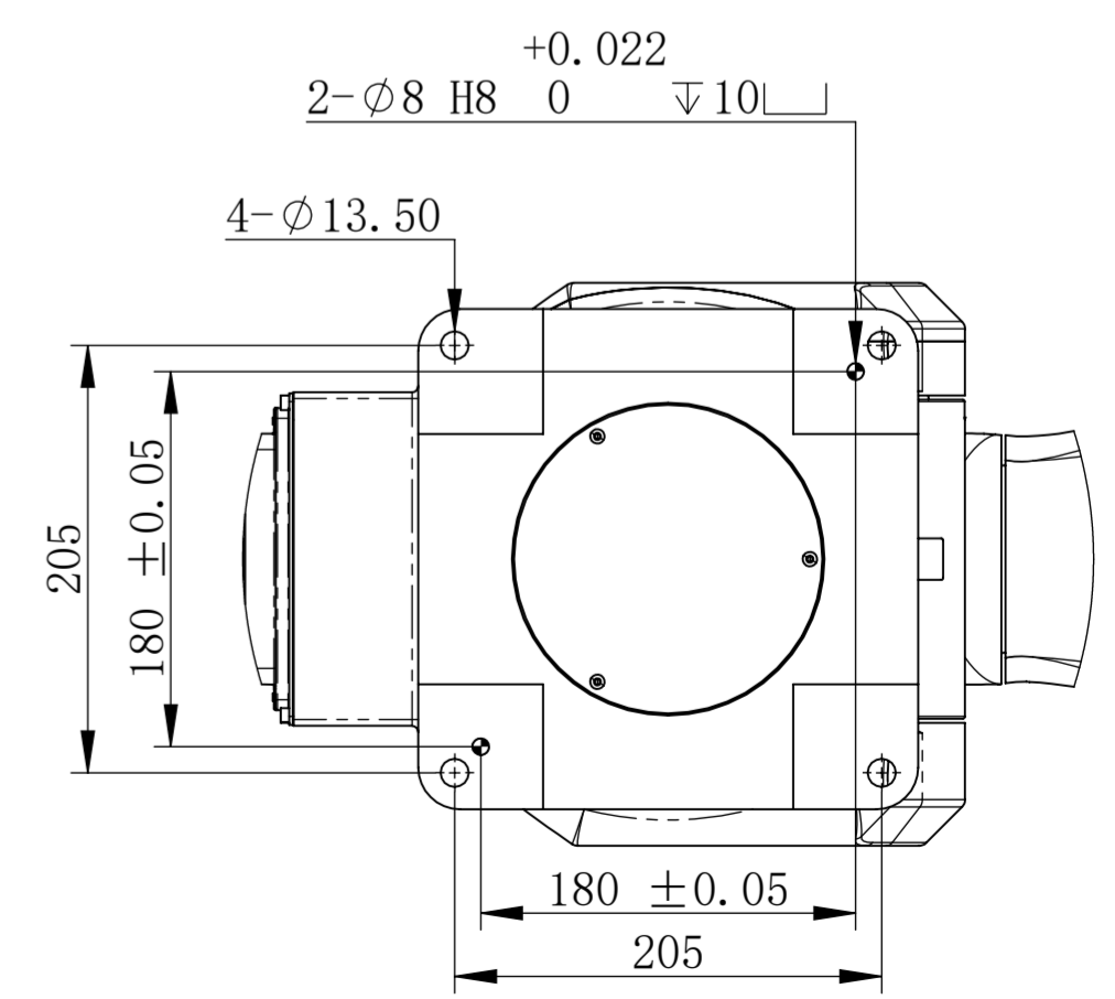
Base Installation Diagram
