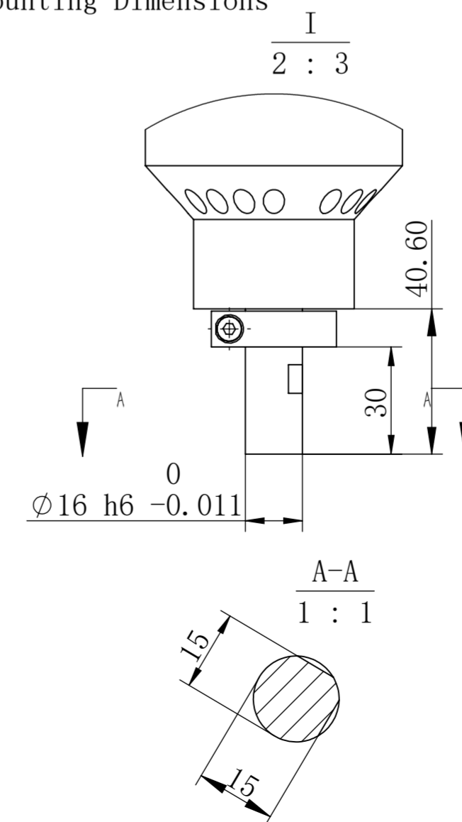
End Mounting Dimensions
