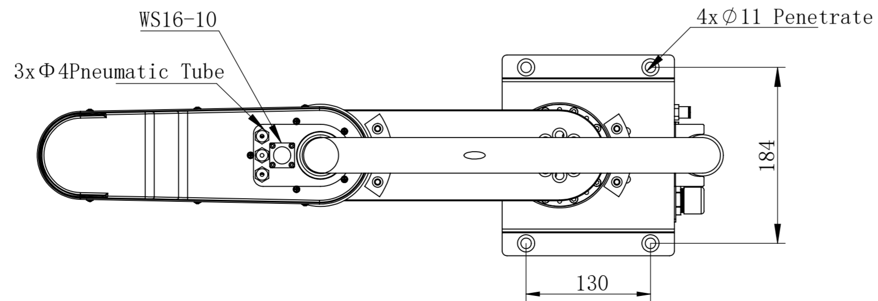
Base Mounting Dimensions
