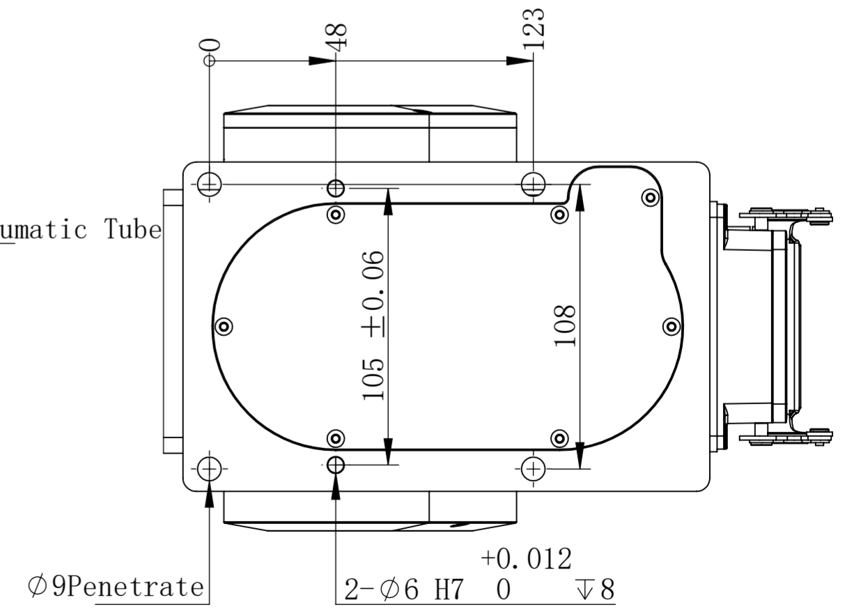
Base Installation Diagram
